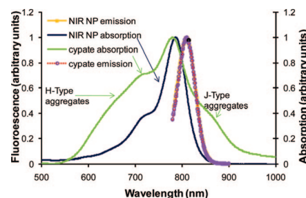
Figure 3. Steady state absorption and emission properties of the infrared imaging agent cypate and the NIR nanoprobes. In buffered aqueous solutions (10% MeOH), cypate may form H type aggregates, while the NIR nanoprobes show diminished aggregation in all the buffers, and organic solutions we tried.
