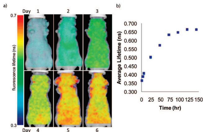
Figure 5. (a) Fluorescence lifetime maps of site-isolated NIR fluorescent nanoprobe in vivo at 1–6 days postinjection. The lifetimes detected are homogeneous for the first hour but gradually begin to increase heterogeneously in a site specific manner. Highest lifetimes are seen in the liver and intestines, likely due to increased metabolism of the nanoprobe. (b) A plot of average measured fluorescence lifetime as a function of time in the liver. The measured fluorescence lifetime in vivo increased over time with a significantly nonzero slope ( p < 0.01 ) of 0.004 ns/h and intercept of 0.35 ns using a linear correlation model of 0–50 h.
